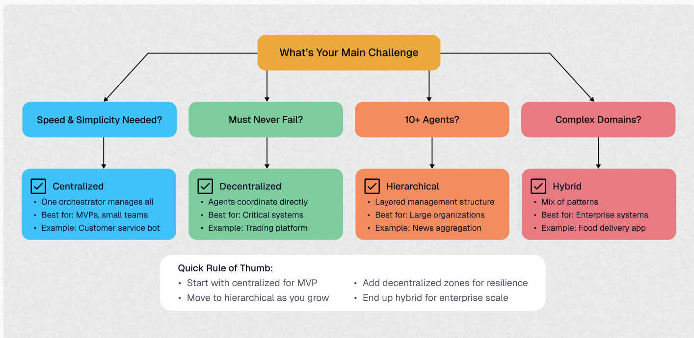
FIGURE 3.6 An architecture decision framework for selecting the right pattern
