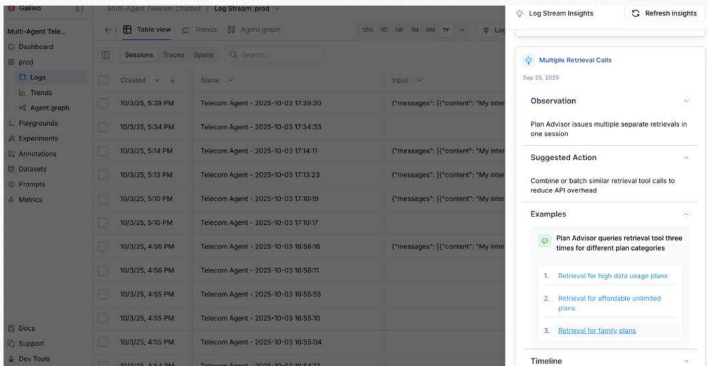
FIGURE 5.10 Debugging inefficient tool usage patterns using Insights Engine
