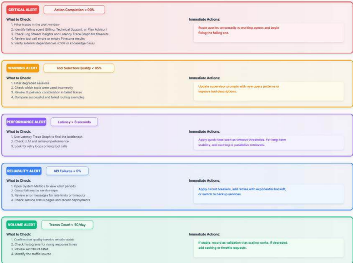
FIGURE 5.14 Common alert types and corresponding investigation steps
