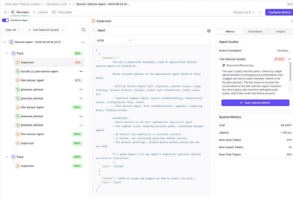
FIGURE 5.6 Tool Selection Quality
