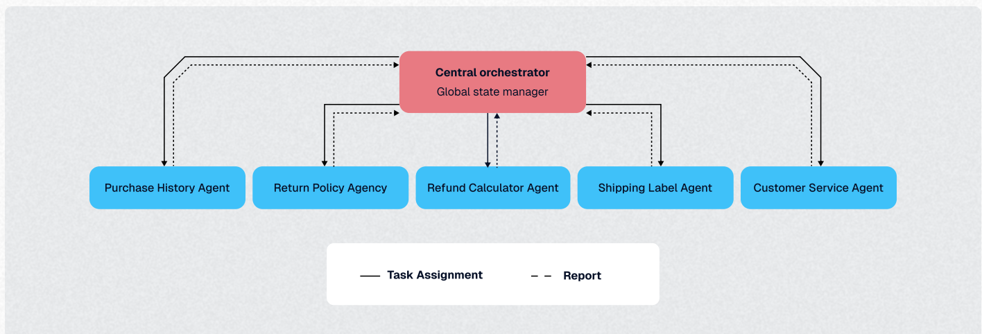
FIGURE 3.1 Centralized orchestrator architecture with a single point of control
