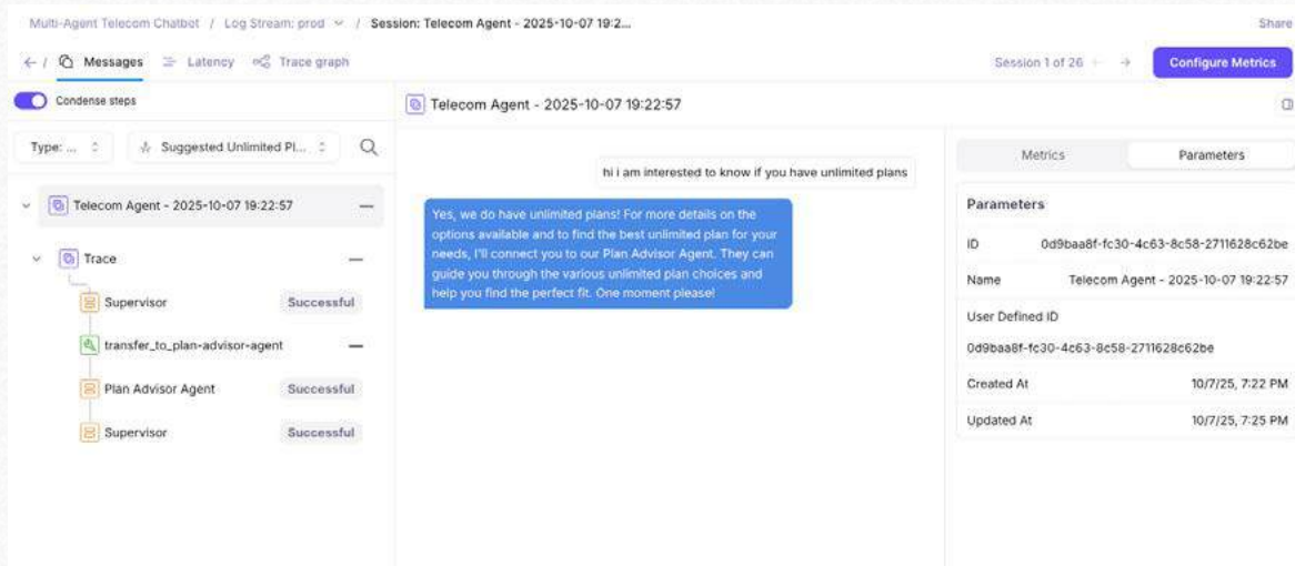
FIGURE 5.12 Evaluating the system behavior
