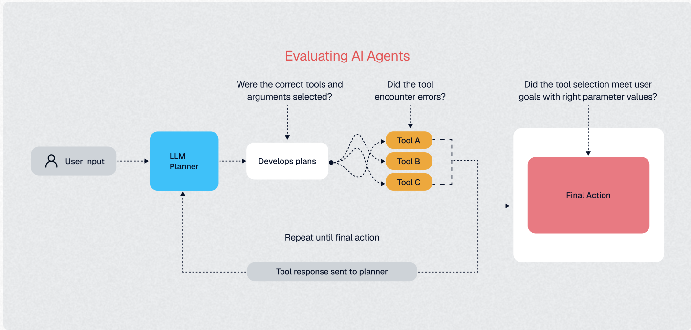
FIGURE 2.4 Tool Selection Scoring
