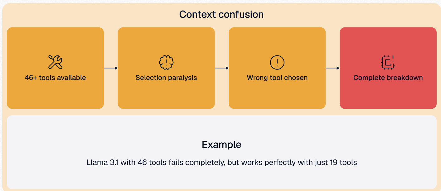
FIGURE 4.4 Context confusion from tool overload to complete breakdown
