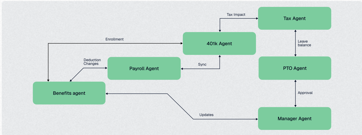
FIGURE 3.2 Decentralized peer-to-peer architecture
