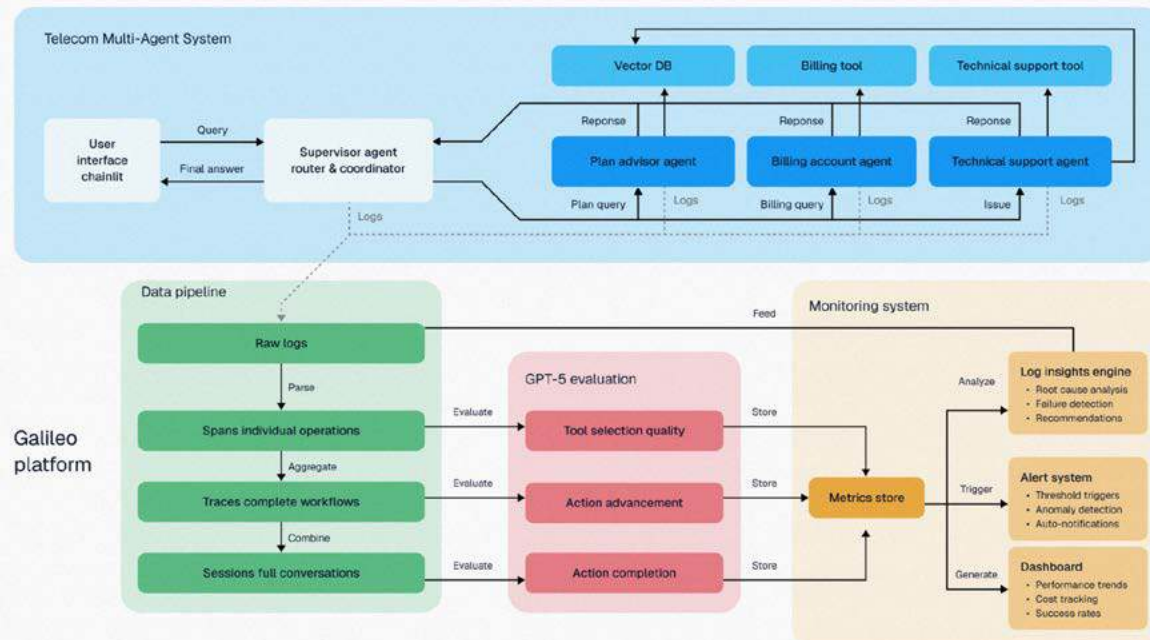
FIGURE 5.1 Telecom multi-agent architecture with observability
