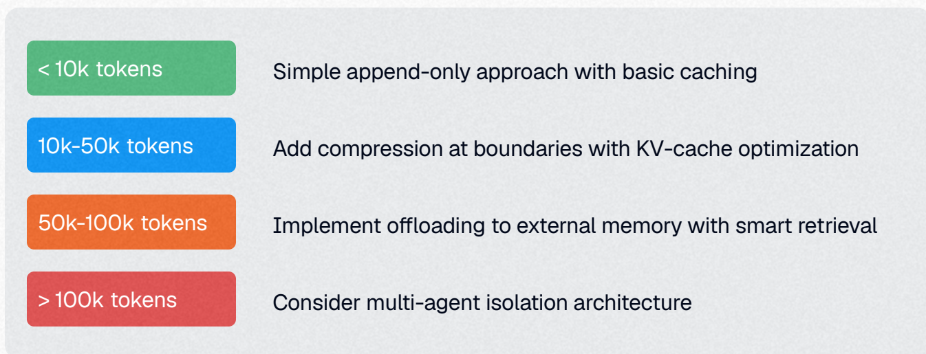
FIGURE 4.6 Context size thresholds and recommended approaches
