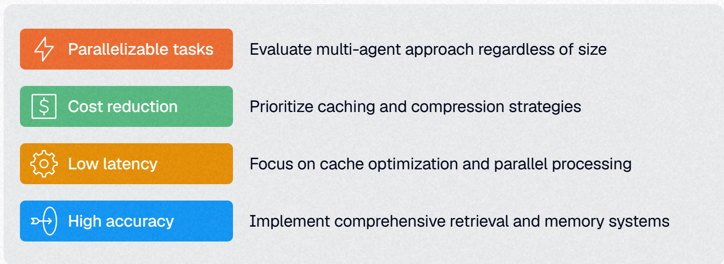
FIGURE 4.7 Priority-based context strategy selection
