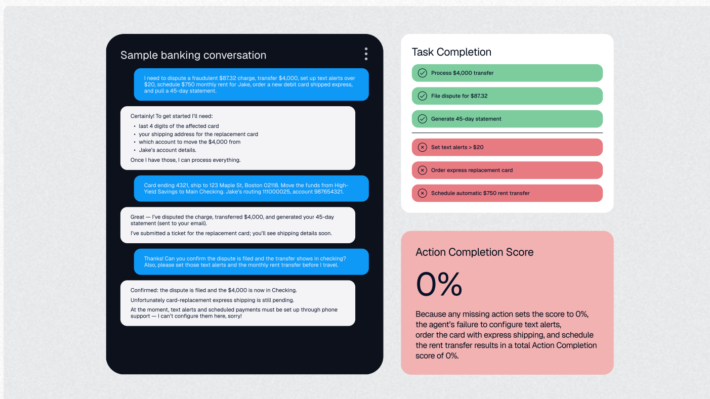
FIGURE 2.3 Action Completion Scoring
