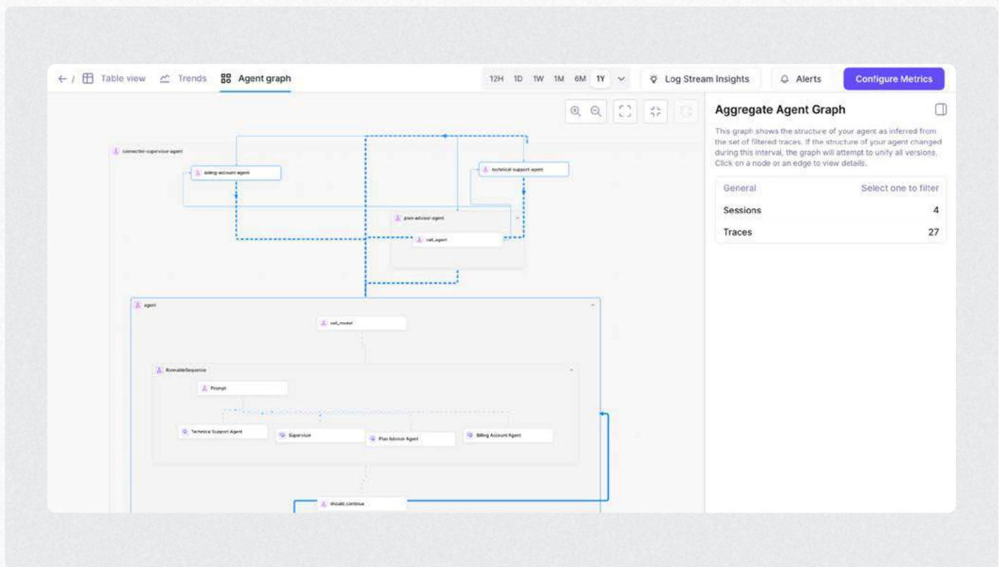
FIGURE 2.7 Graph View
