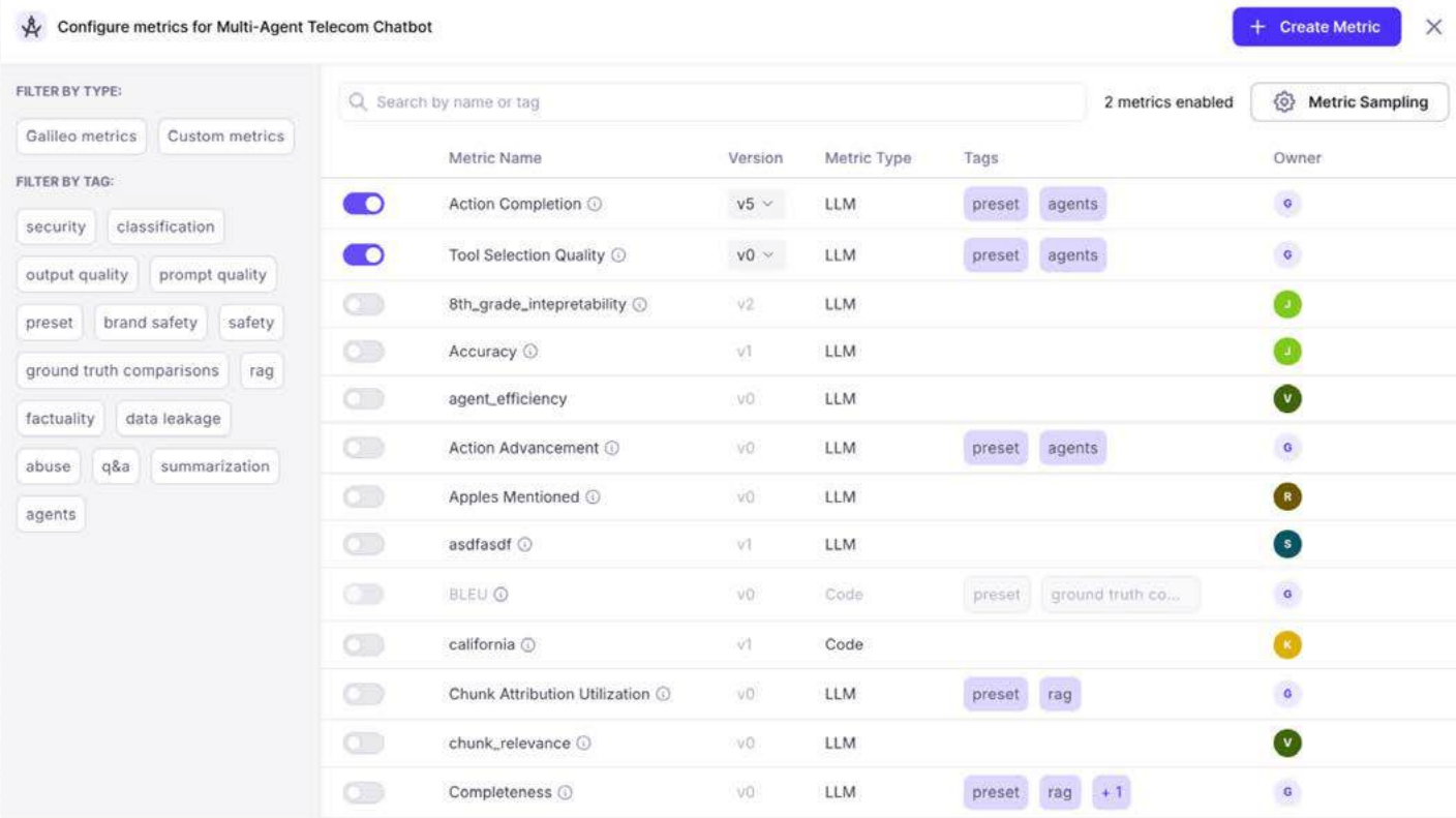
FIGURE 5.5 Configure Metrics
