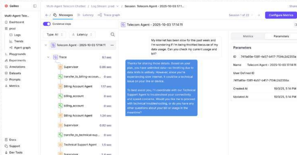
FIGURE 5.3 Galileo's console for observability
