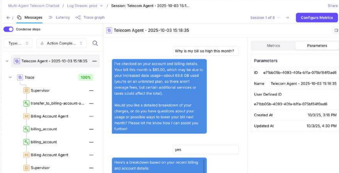
FIGURE 5.4 Action Completion step
