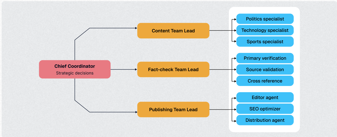
FIGURE 3.3 Hierarchical multi-level architecture with specialized teams
