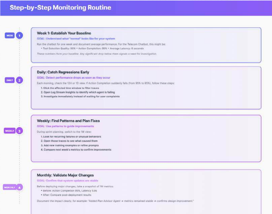
FIGURE 5.13 Step-by-step monitoring
