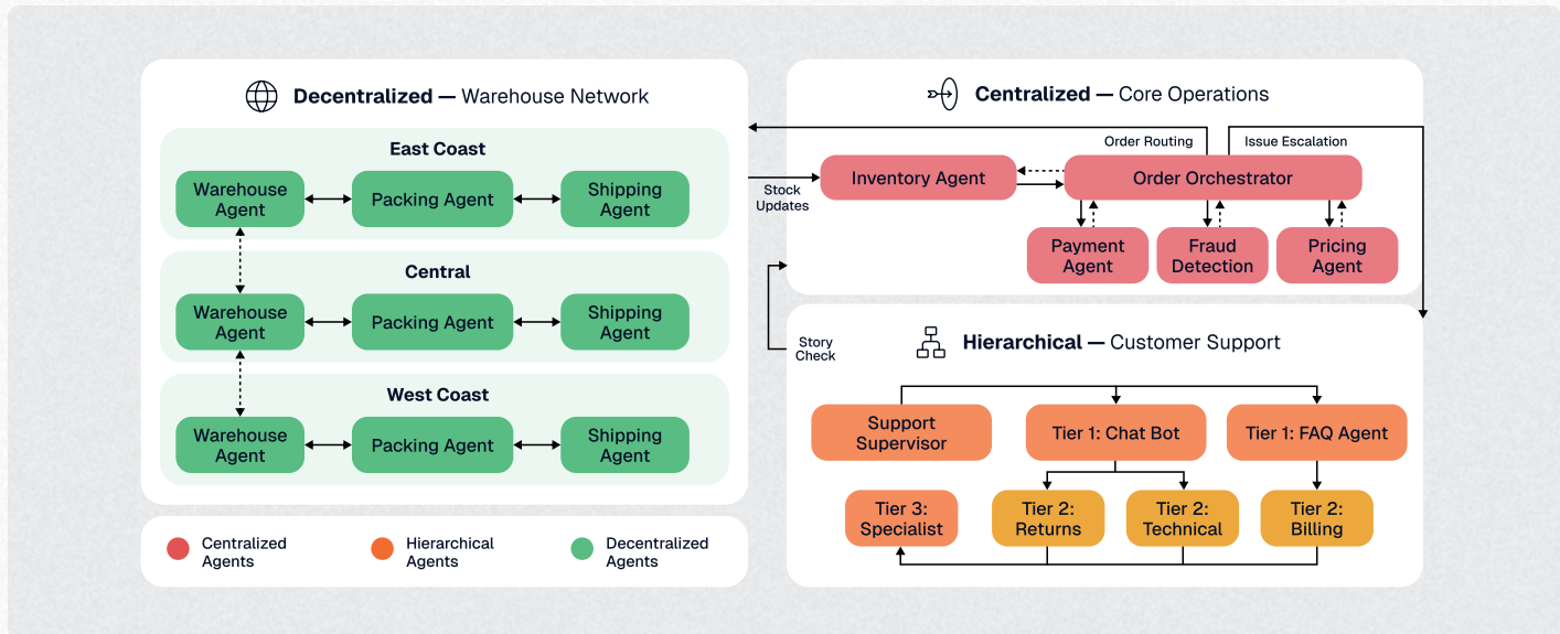
FIGURE 3.4 Hybrid architecture
