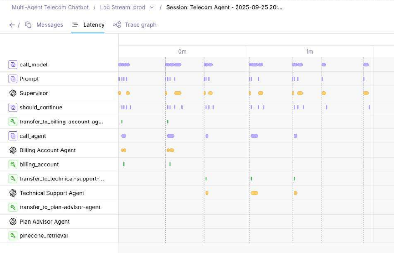
FIGURE 5.8 Timeline View
