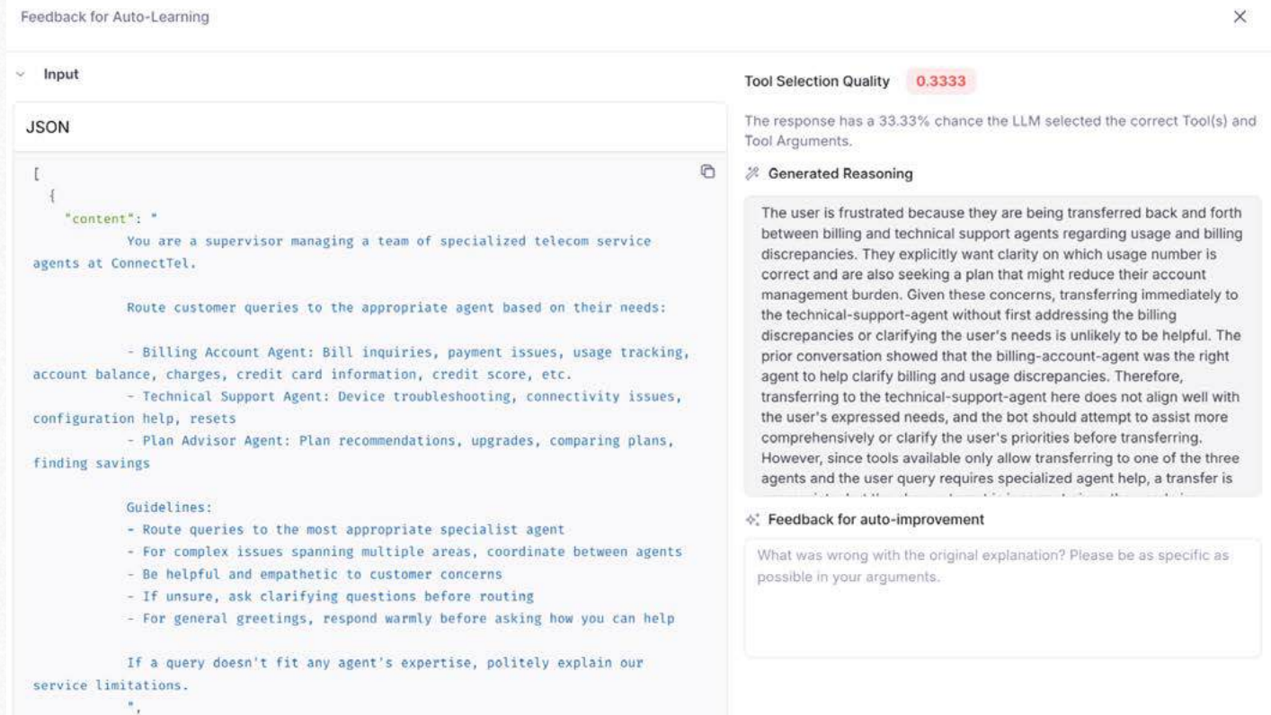
FIGURE 5.7 Metric Explanations
